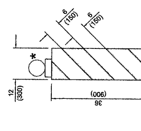
VERTICAL BARRICADE
