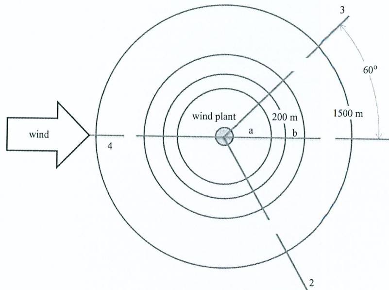
Fig. 1. Scheme of vibration, noise and infrasound measurements around the wind plant: 1, 2, 3, 4 – measuring directions; a – the diameter of the first circle resulting from PN-EN 61400-11; b – distance between following circles (100 m).
